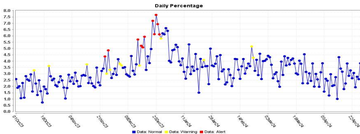
Figure 12. Percentage of ED and UC* Visits for ILI for Weeks 40-17, Washoe County, 2023-2024
